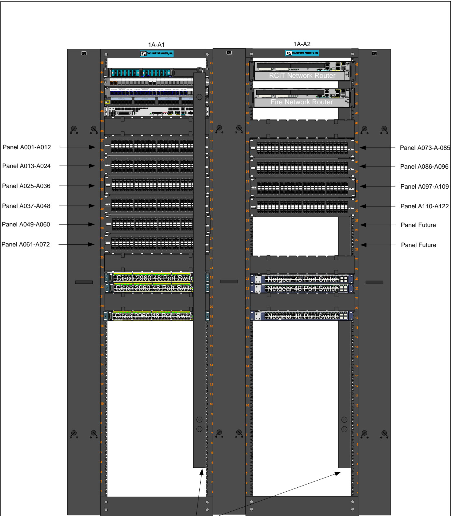
APC Vertical PDU #AP7930 15 Amp Nema 5-15P (10) 5-20R
