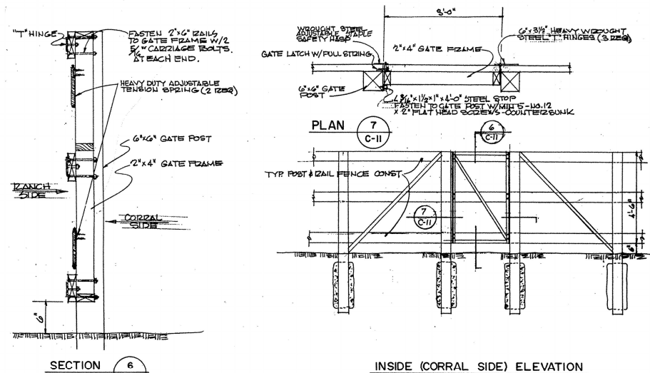
5'-0" HIGH TYPE "C" (CORRAL SIDE) FENCE & GATE DETAILS N.T.S. (8) C-10
