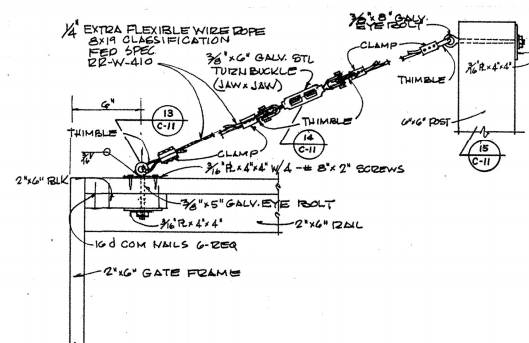
GATE SUPPORT DETAILS N.T.S.
