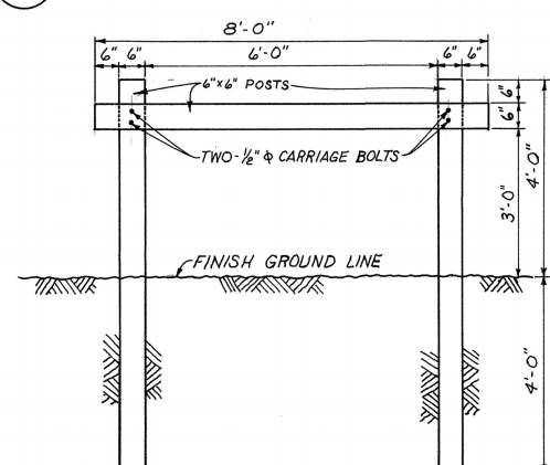
HITCHING RAILS SCALE 1" = 2' (10) C-10
