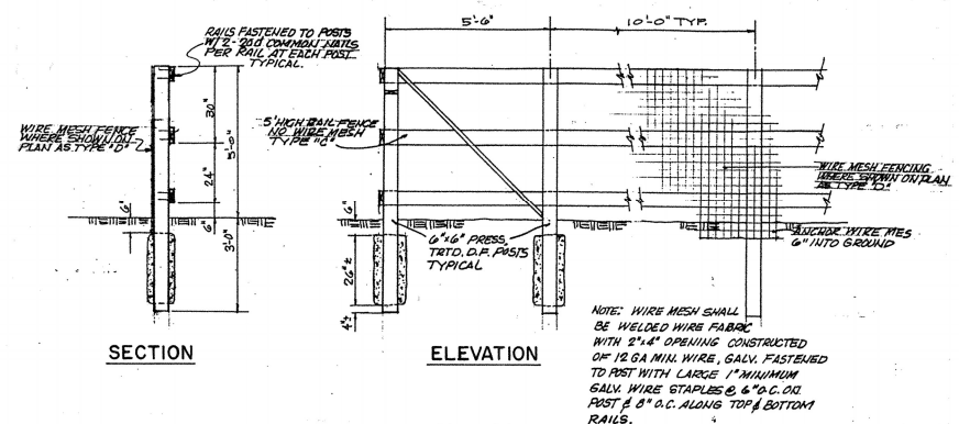
5'-0" HIGH TYPE "D" FENCE DETAILS N.T.S. (4) C-10
