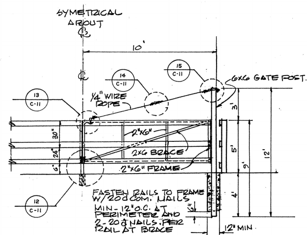
20' DBL. SWING WOOD GATE DETAIL N.T.S. (11) C-10
