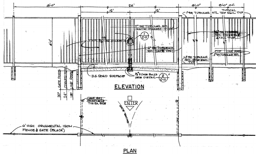
FENCE TYPE "B" ORNAMENTAL IRON FENCE & GATE DETAILS N.T.S. (3) C-10
